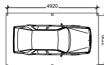
Carport
